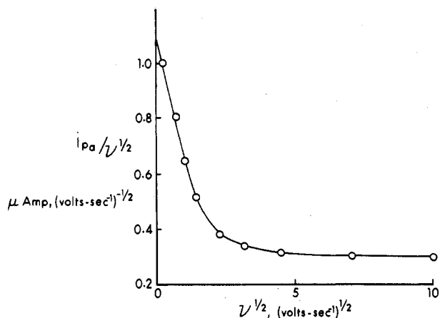
Figure 2. Dependence of i_{pa}/\nu^{1/2} as a function of \nu^{1/2} in the electrochemical oxidation of 1.0 \times 10^{-3} M \text{Fe}(\text{GMI})_3^{2+} in 0.5 \text{ M H}_2\text{SO}_4 on a glassy carbon working electrode at 25^\circ\text{C} .
