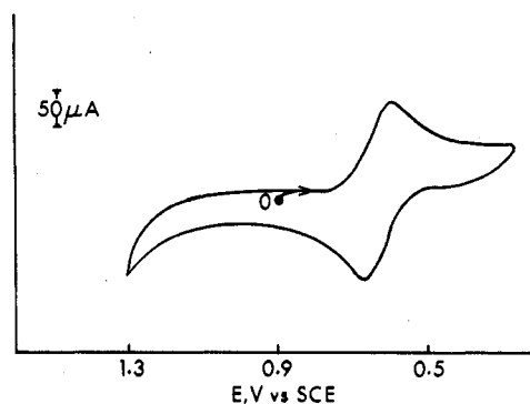
Figure 4. Cyclic voltammogram of a 8.9 \times 10^{-4} M solution of \text{Fe}(\text{GMI})_2(\text{GA})^{3+} , obtained in the oxidation of a 1.2 \times 10^{-3} M solution of \text{Fe}(\text{GMI})_3^{2+} by 4.5 equiv of \text{Ce}(\text{IV}) , in 0.5 \text{ M H}_2\text{SO}_4 .
