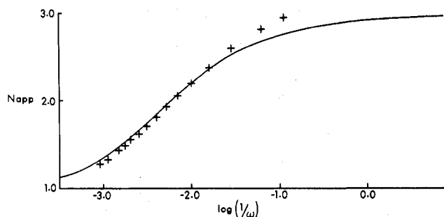
Figure 8. Plot of N_{app} vs. \log(1/\omega) . Solid line shows calculated curve using k = 22 \pm 2 \text{ s}^{-1} , D = (8.0 \pm 0.8) \times 10^{-6} \text{ cm}^2 \text{ s}^{-1} , and \nu = 0.011 \text{ p} . Plus signs show the experimental data obtained from rotating-disk studies. Each experimental point is an average of six determinations on four different complex concentrations.
